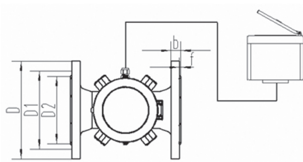
SCL-61D Ultrasonic Water Meter (Metal Casing) (DN50~DN300)
