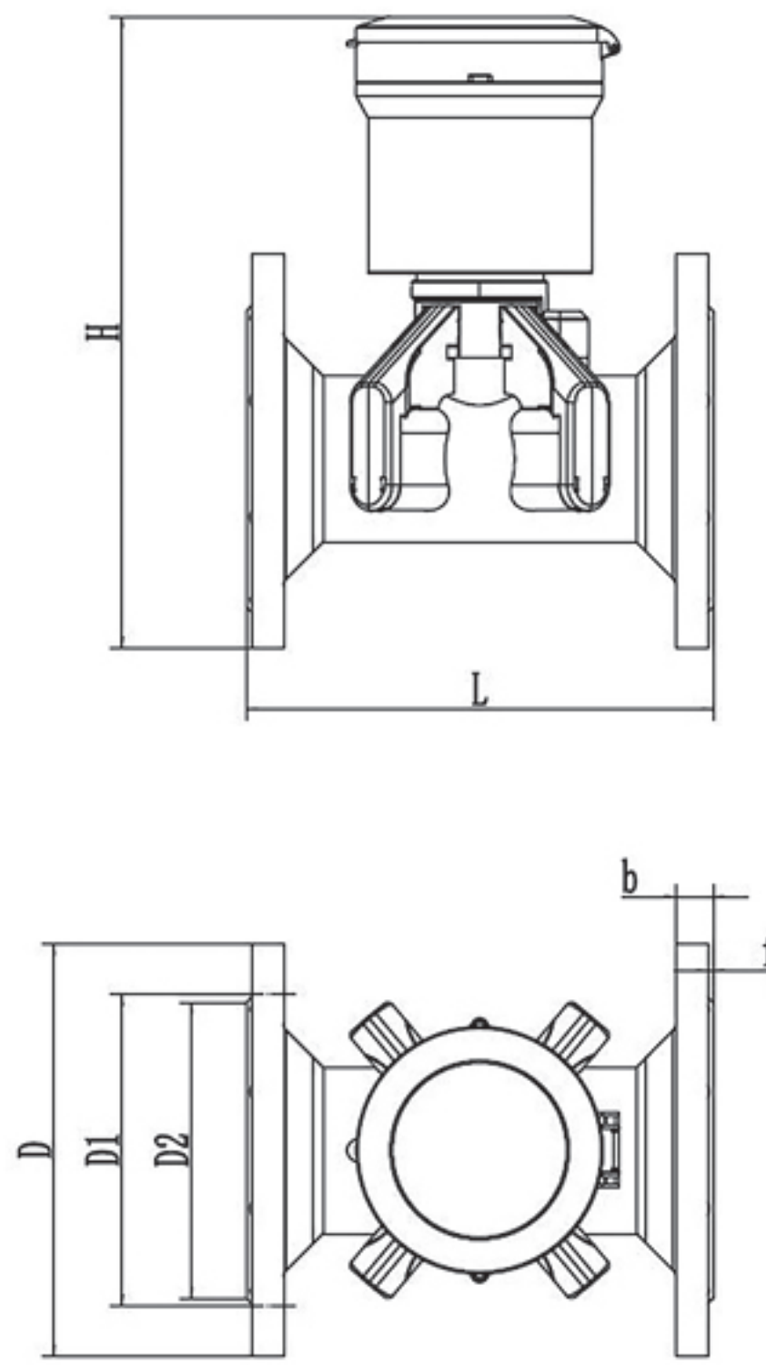
SCL-61D Ultrasonic Water Meter (Metal Casing) (DN50~DN300)
