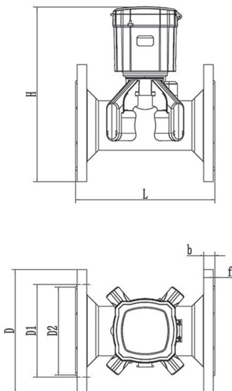
SCL-61D Ultrasonic Water Meter (Plastic Casing) (DN50~DN300)
